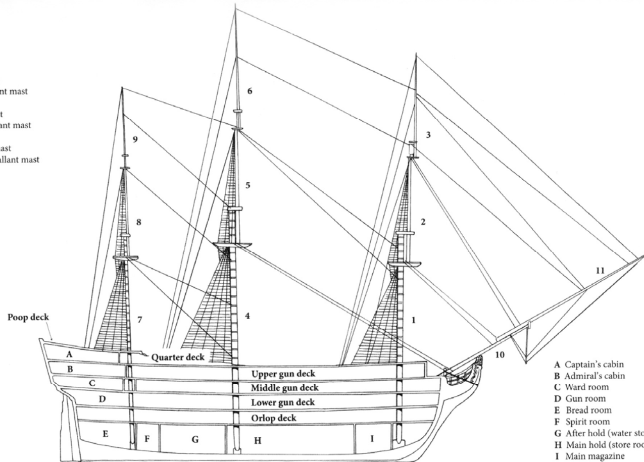
The standing rigging, masts and decks of a 100-gun ship of the line
